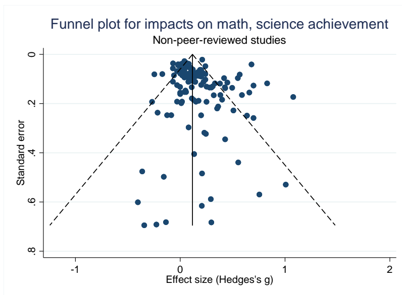
Figure A1. Funnel plot of included effect sizes.
